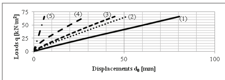
Fig. 5b. Displacements d_0 (mm) depending on the use of sheet piles as a cover of the foundation. Vertical load applied on the backfill of road embankment
