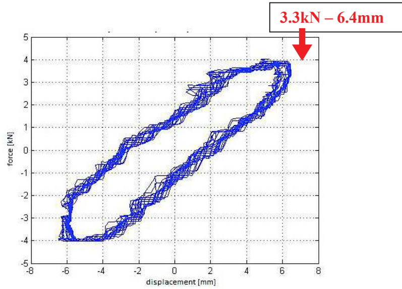
Figure 8. Hysteresis loop – maximum displacement and corresponding force
