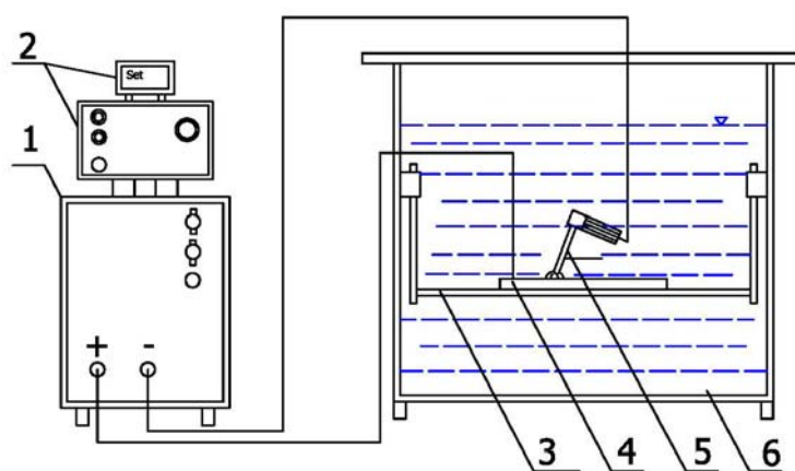
Fig. 1. Test stand for underwater wet welding: 1) welding power source, 2) control panel, 3) table, 4) plate, 5) electrode, 6) tank
