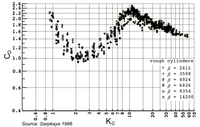
Fig. 7. Comparison of drag coefficient C_D for six rough cylinders, k/D=50 . Source: Sarpkaya [2]
