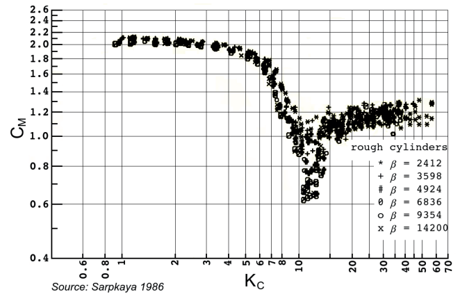
Fig. 6. Comparison of inertia coefficient C_M for six rough cylinders, k/D=50 . Source: Sarpkaya [2]
