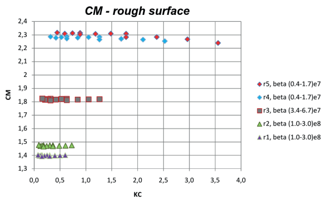
Fig. 15. A graph of the C_M as a function of K_C for the subsequent segments of the structure. Rough surface
