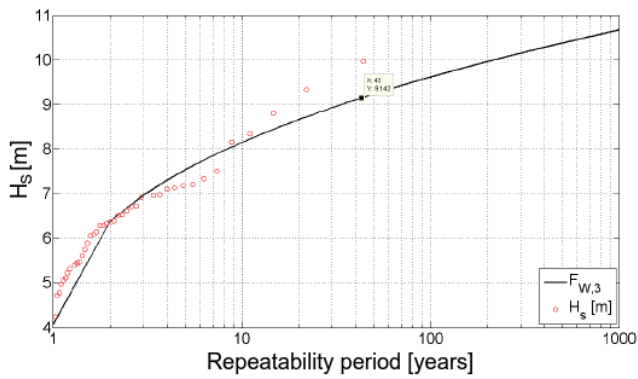
Fig. 2. Significant wave height H_s as a function of return period. Weibull distribution for location: 7,750 E, 55,50 N (Baltic Sea – Polish economic zone)
