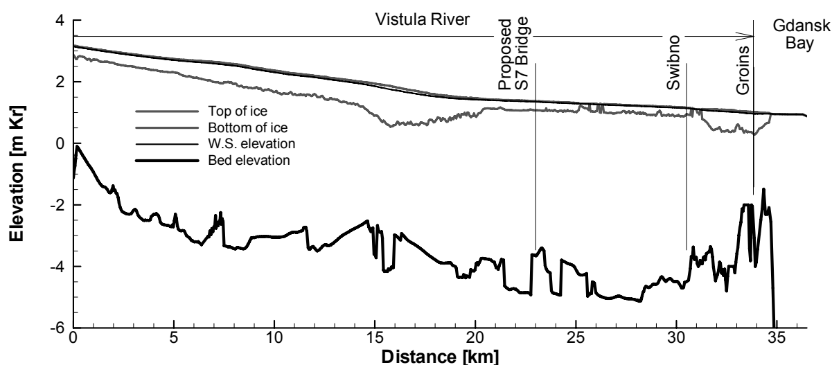
Figure 7. Longitudinal profile of water surface elevation and ice thickness for case 8 (low discharge in the river, 100 year storm in the Gdańsk Bay and high wind velocity).
