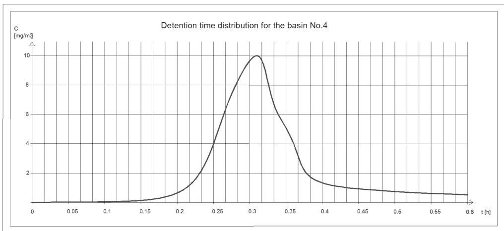
Fig. 3. Retention time distribution for pool No. 4
