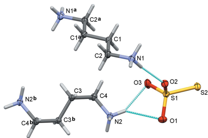
Figure 4 Molecular structure and atom-labelling scheme of 1,4-butylenediaminium thiosulfate (3), symmetry operation codes: ( a ) -x + 1, -y, -z + 1 ; ( b ) -x + 1, -y, -z . Hydrogen bonds shown as dotted lines. Hanging hydrogen bonds are deleted. Ellipsoids drawn at the 50% probability level.
