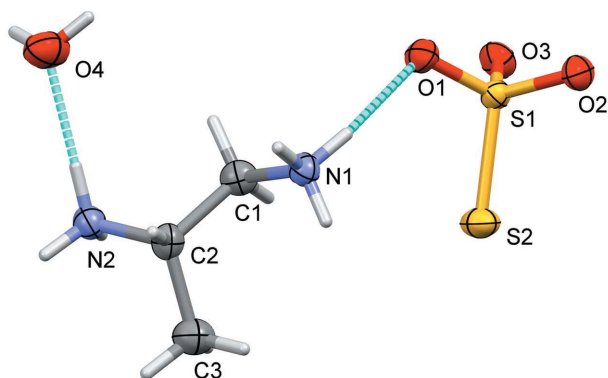
Figure 1 Molecular structure and atom-labelling scheme of 1,2-propylenediaminium thiosulfate (1 a ). Hydrogen bonds shown as dotted lines. Hanging hydrogen bonds are deleted. Ellipsoids drawn at the 50% probability level.
