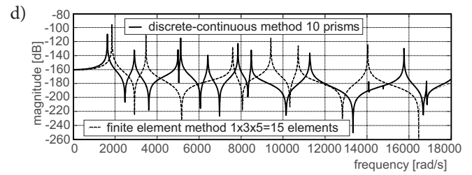
Fig. 7. Frequency characteristics
