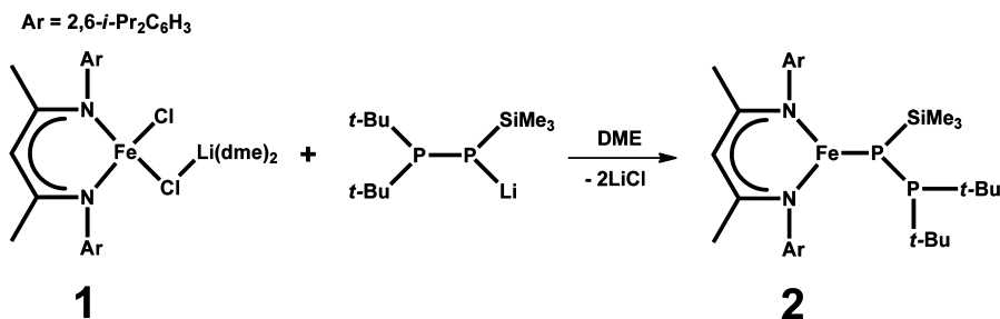
Scheme 3. Synthesis of the Side-On Phosphanylphosphido Complex 3
