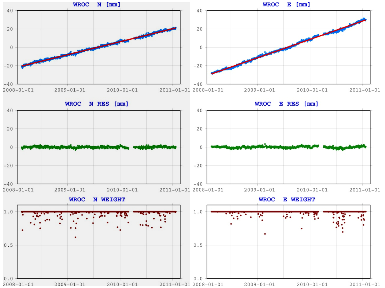
Fig. 9 Trend line (velocity) determination for WROC (Wrocław, PL) GPS site. From top: time series and trend line, residuals after trend line removal and weights for particular coordinates determined using robust estimation.
