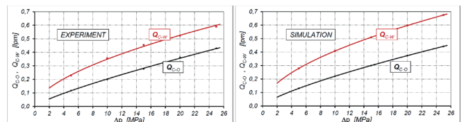
Fig. 19. Characteristics of Q_{C,W}=f(\Delta p) experimentally obtained (left) and calculated from equations (39) and (40) (right).
