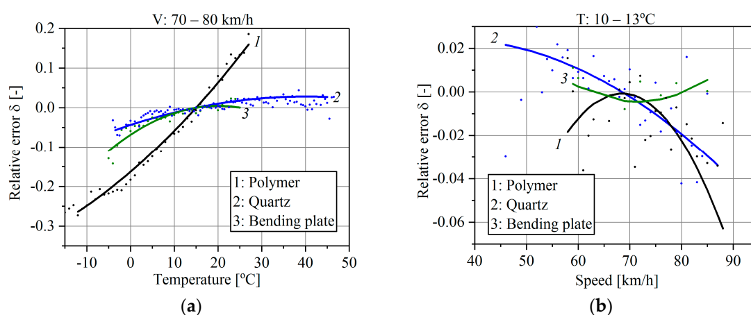
Figure 4. (a) Temperature characteristics; (b) Speed characteristics of polymer, quartz and bending plate sensors installed in the pavement.
