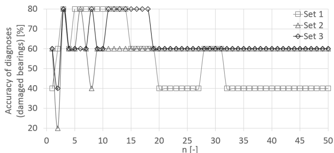
Fig. 2. Graph of accuracy of diagnoses for damaged bearings.
