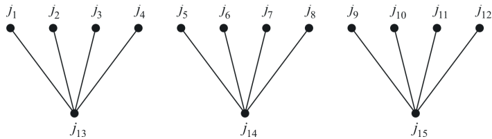
Fig. 4. Example of incompatibility graph G = 3K_{1,4}
