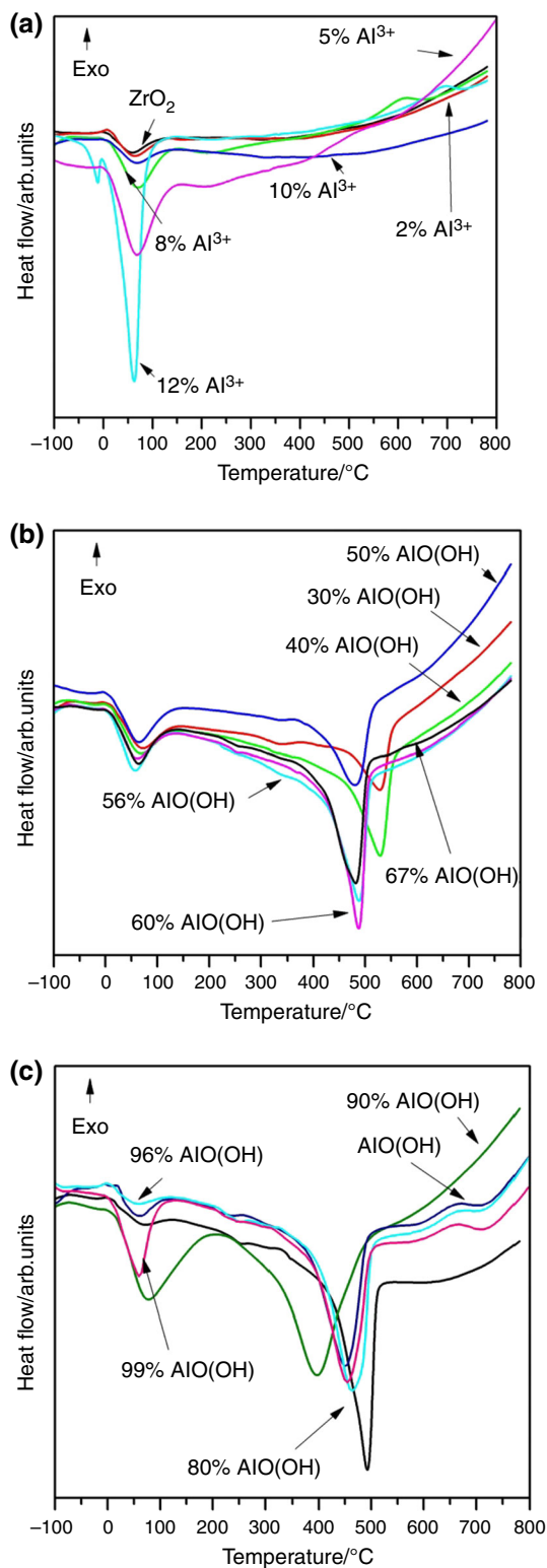
Fig. 5 LT-DSC curves for \text{ZrO}_2 with different \text{AlO}(\text{OH}) content, where a shows 100% \text{ZrO}_2 , and \text{ZrO}_2 with 2–12% of \text{Al}^{3+} addition, b \text{ZrO}_2 with 30–67% of \text{AlO}(\text{OH}) additive and c represents 100% \text{AlO}(\text{OH}) , and \text{ZrO}_2 with 80–99% of \text{AlO}(\text{OH}) additive
