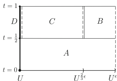
FIGURE 3. Partition of I \times U^\epsilon
