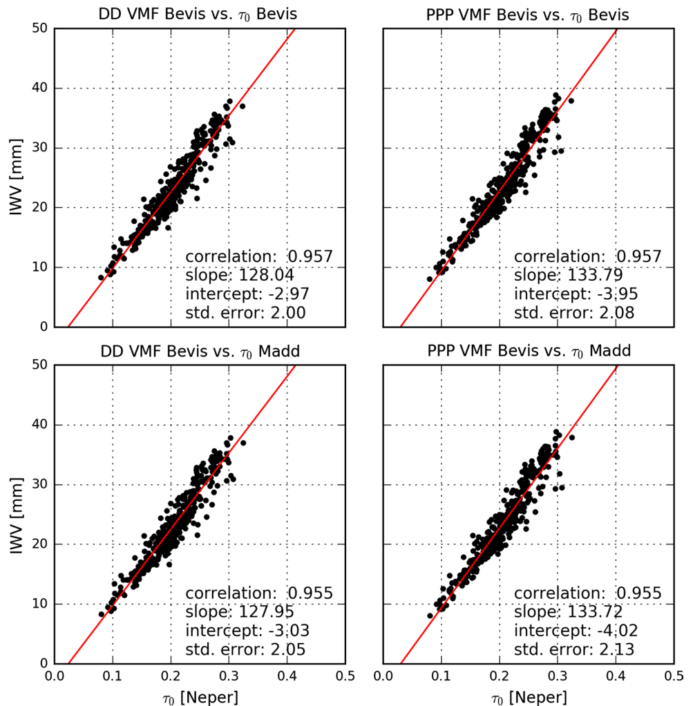
Fig. 10 Correlation between IZW and \tau_0 derived from GNSS processing using VMF1
