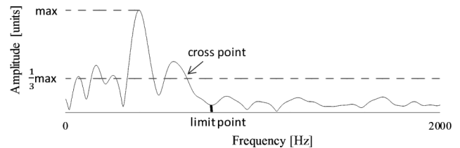
Fig. 2. The magnitude response of the phoneme /k/.
