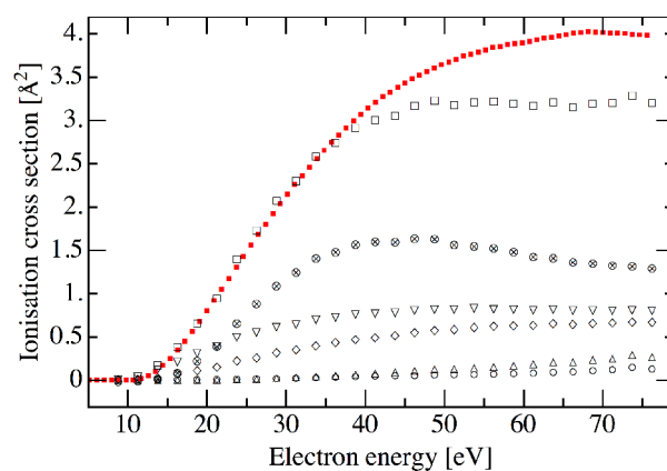
Fig. 5. (a) (□) The total ionization cross section of formic acid molecules derived from the partial ionization cross sections of the (⊗) \text{COH}^+ , (∇) \text{HCOOH}^+ , (◇) \text{COOH}^+ , (Δ) \text{CO}^+ and (○) \text{CO}_2^+ + \text{OH}^+ + \text{O}^+ cations obtained at 70 eV; (b) the total ionization cross section (■) from the total ion collection experiment (Sect. 2.1).
