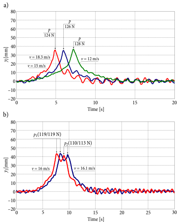
Fig. 11. Comparison of measurement results of contact wire uplift waveform for: a – locomotive with the same raised pantograph p with small variations in speeds, registered in subsequent days; b – suburban train with two raised pantographs p_1, p_2 spaced at l_{1-2} = 24 m, with equal speeds, registered twice on the same day
