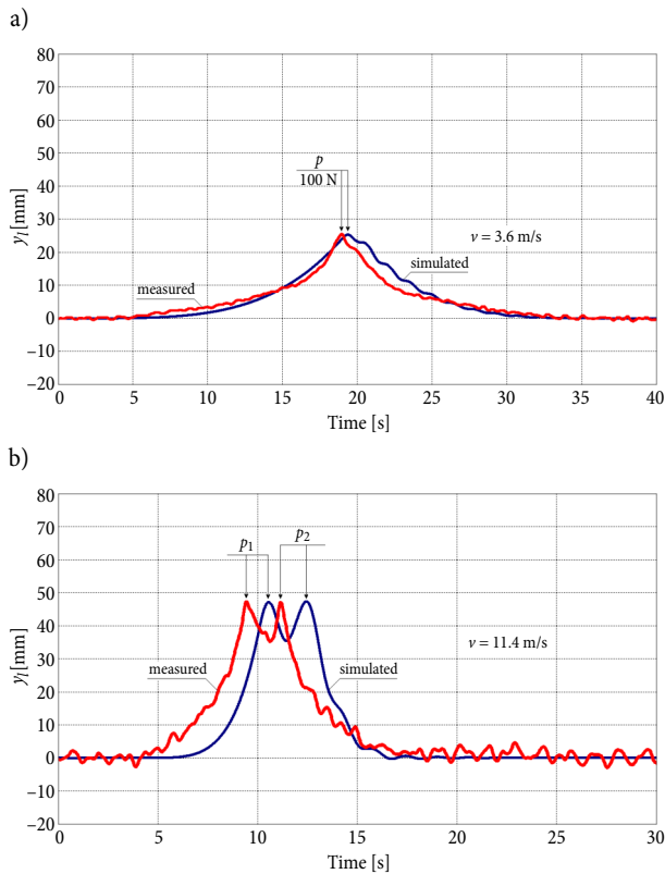
Fig. 9. Comparison of simulation and measurement results of contact wire uplift waveform for: a – train with one raised pantograph p of static force F_u = 100 N; b – train with two raised pantographs p_1, p_2 spaced at l_{1-2} = 24 m of static force F_{u1} = F_{u2} = 130 N
