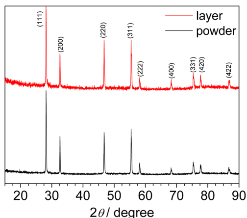
Fig. 2 XRD patterns of \text{Bi}_3\text{YO}_6 for the powder sample and deposited layer
