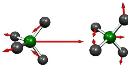
FIG. 1. (Color online) Pictorial representation of the two antisymmetric vibrational modes of CF 4 which we are considering in the present work: on the left we show the stretching mode \nu_3 while on the right we represent the bending mode \nu_4 .
