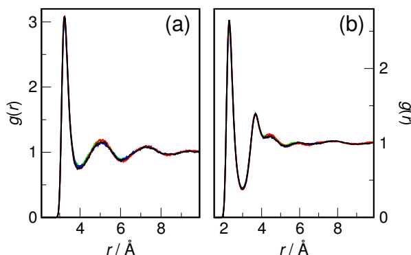
Figure S1: Radial distribution functions, g(r) , for (a) Cl \cdots O and (b) Cl \cdots H pairs in the studied Cl - (H 2 O) n systems for n = 64 (green), 128 (blue), 256 (red), and 512 (black).
