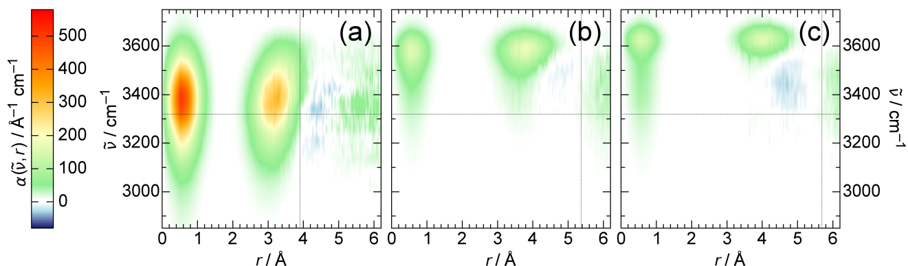
Figure 5: Radially-resolved IR spectra, eq 15, in the water OH stretching vibrations range for (a) \text{Cl}^- , (b) \text{BF}_4^- and (c) \text{PF}_6^- . Thin horizontal lines indicate the band position at maximum for bulk water, while thin vertical lines show the extent of the first hydration shells as inferred from the first minima in g_{\text{XO}}(r) (see Figure 1).
