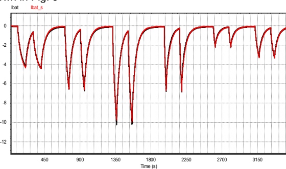
Fig. 13. Comparison of current response i_{bat_s} of the hybrid storage model and real response i_{bat} to the identical load profiles i_{load} as shown in Fig. 9
