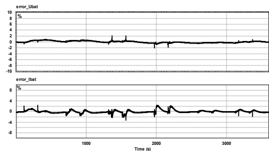
Fig. 11. Voltage and current response errors on the pulsed i_{load} current load
