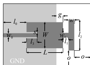
Fig. 20. Geometry of the dual-band patch antenna [18]. Ground plane marked using the lighter shade of gray.
