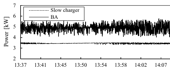
Fig. 5. EV Charging with stationary battery pack (BA) via slow charger – fragment.
