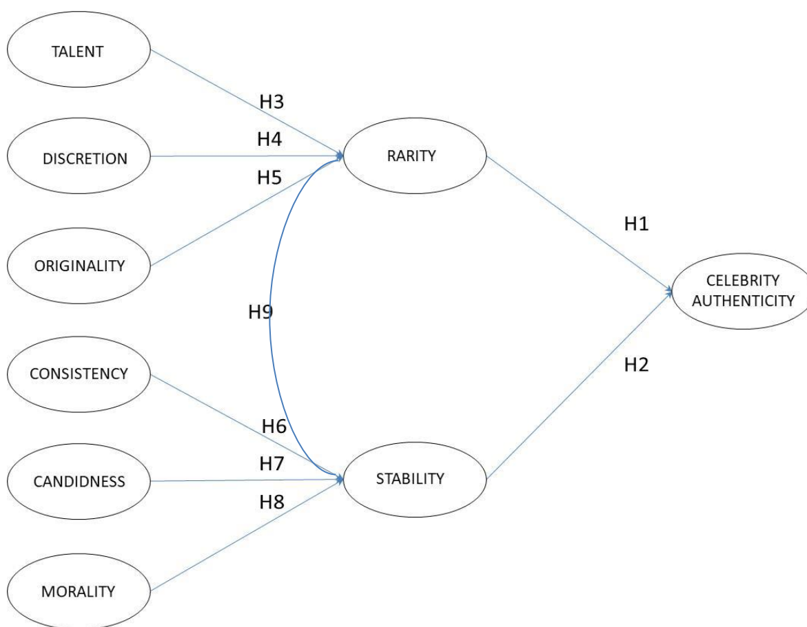
Figure 1: Conceptual framework
