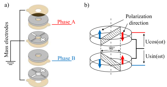
Fig. 3. Piezoceramics arrangement in single actuator of MPM.
