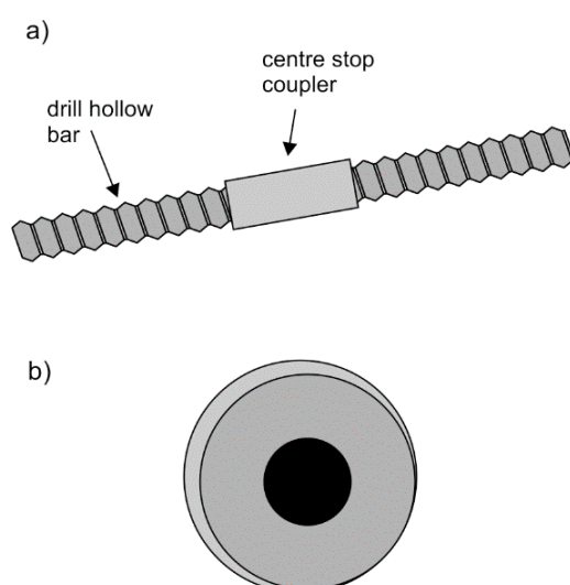
Figure 7.1 Scheme of self-drilling systems of ground anchors: a) two drill hollow bars connected by the centre stop coupler, b) cross-section of the bar
