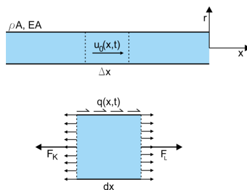
Figure 2.1 Differential element of a rod with loads
