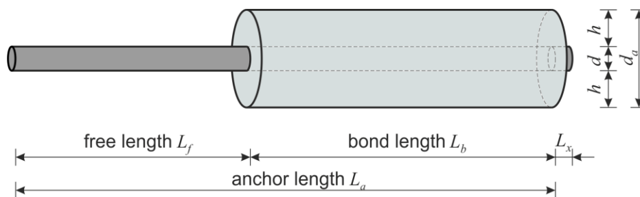
Figure 4.7. Geometry of the laboratory model of ground anchor
