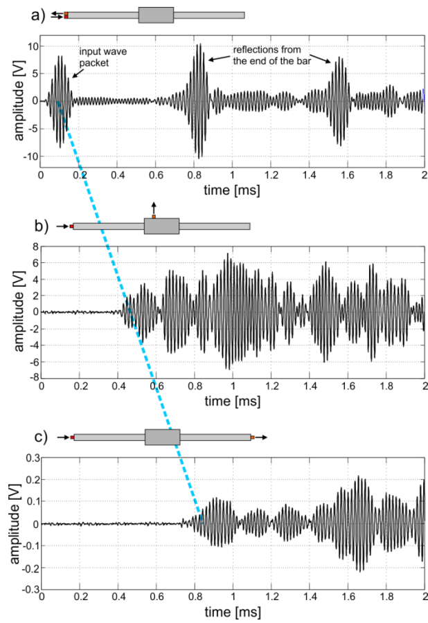
Figure 7.10 Wave propagation signals registered at the self-drilling hollow bar system: a) signal registered at the beginning, b) at the coupler in the middle and c) at end of the bar
