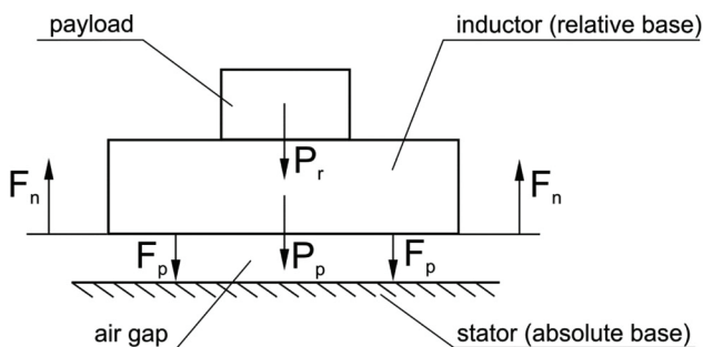
Figure 3. Forces of precise coordinate positioning system.
