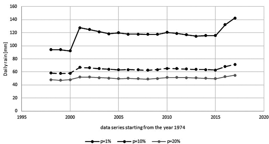
Fig. 3. Maximum theoretical daily rain sum with the probability of exceedance of 1%, 10% and 20% according to the log-normal distribution with maximum likelihood estimation (MLE)
