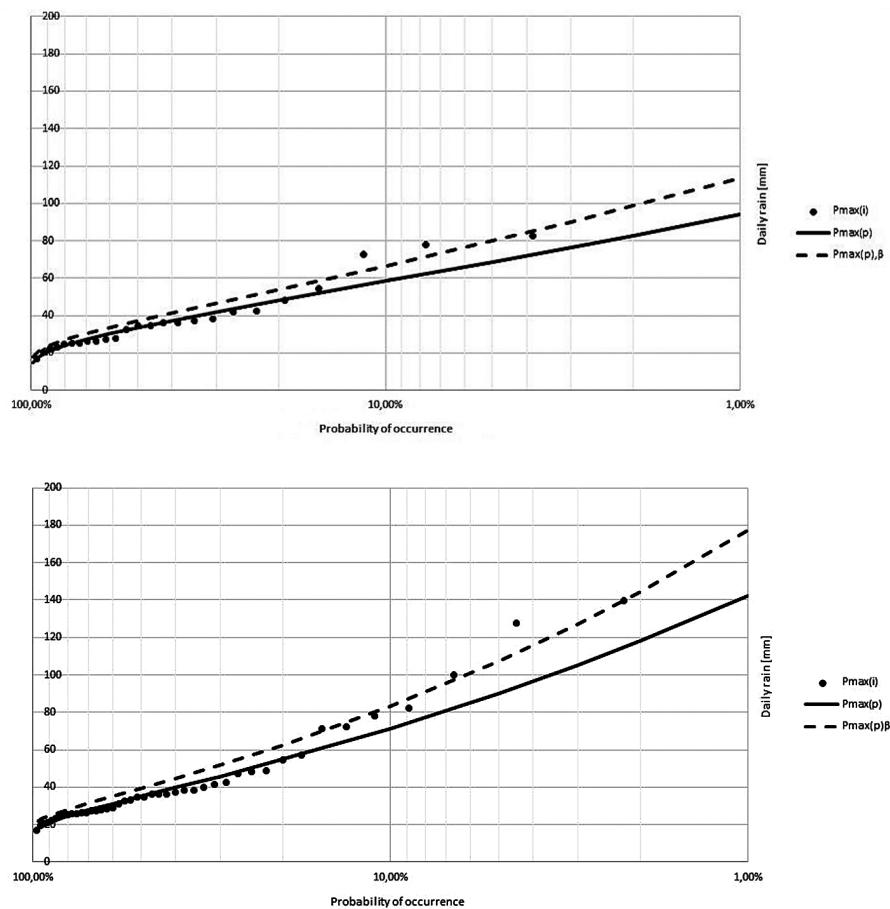
Fig. 2 The maximum annual sum of daily rainfall observed at the station of Gdańsk Rębiechowo in the periods of (1974–1998) and (1974–2017). The curve of probability of exceedance according to the log-normal distribution with maximum likelihood estimation (MLE) and the limit of 85% confidence interval – P_{\max(p)\beta} . P_{\max(i)} denoting empirical probability of the occurrence of annual maximum daily rain, P_{\max(p)} denoting theoretical probability of the occurrence of annual maximum daily rain
