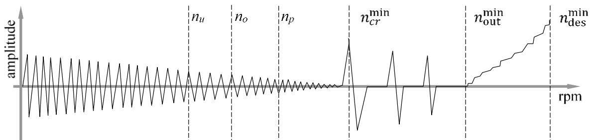
Fig. 1. Characteristic rotational speeds of the circular saw blade according to Stakhiev [17]: n_u – universal; n_o – optimal; n_p – permissible; n_{cr}^{\min} – the lowest critical; n_{out}^{\min} – the lowest self-excited; n_{des}^{\min} – destructive
