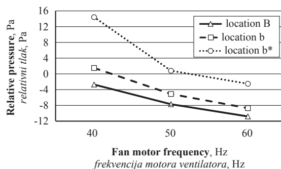
Figure 6 Relative static pressure as a function of fan motor frequency at different locations for wide and narrow cover of the hood; saw blade No. 1 (Ø300 mm), rotational speed 6000 min -1
