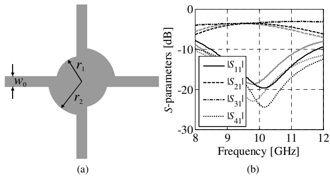
Fig. 2. Initial design of the coupler: (a) topology and (b) frequency characteristics before (gray) and after (black) optimization.
