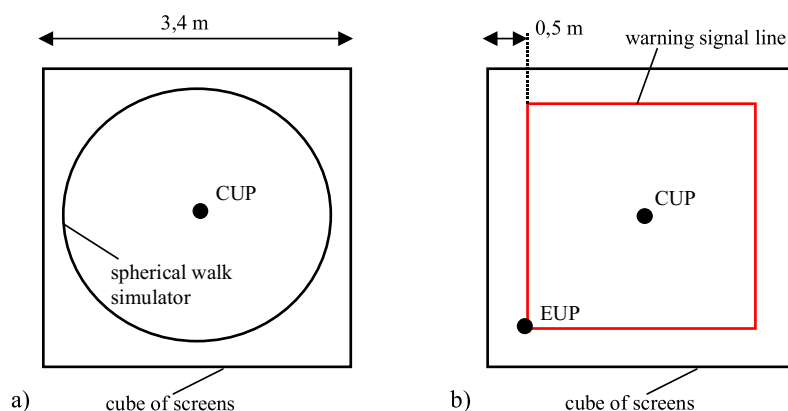
Fig. 5. 13DVL configuration: a) spherical walk simulator is placed into the CAVE, b) “classic” CAVE; CUP – central user position, EUP–extreme user position.
