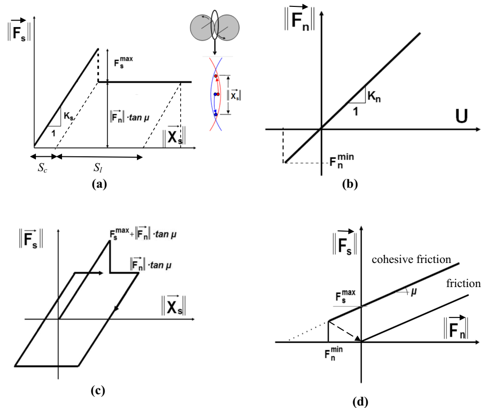
Fig. 2 Mechanical response of DEM: a tangential contact model, b normal contact model, c loading and unloading path in tangential contact model and d modified Mohr–Coulomb model [45, 46]
