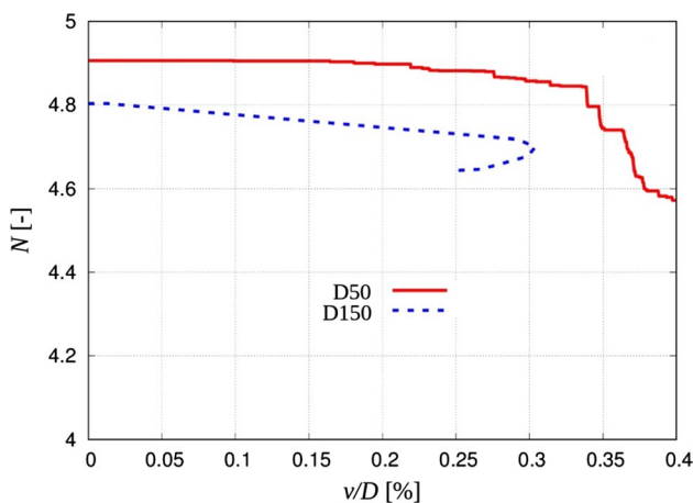
Fig. 11 2D DEM results: evolution of coordination number N versus normalized vertical displacement v/D for two different specimen diameters: D=0.05 m (D50) and D=0.15 m (D150)
