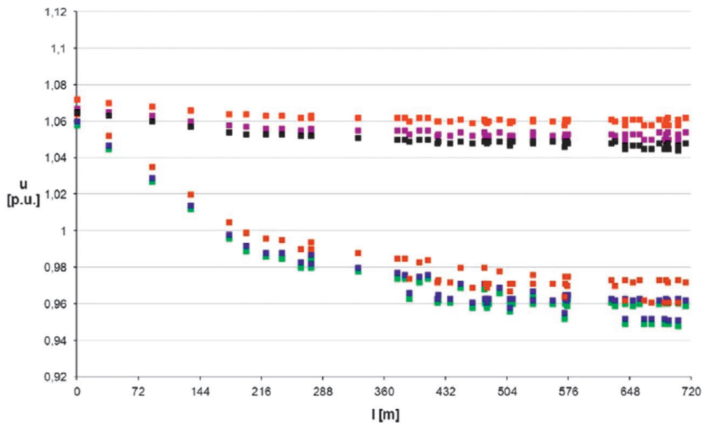
Fig. 8. Voltages with various regulation methods, wind farms output at 30% of rated power: maximum grid load ■ no regulation, ■ regulation by micro-sources, ■ regulation by compensators; minimum grid load – ■ no regulation, ■ regulation by micro-sources, ■ regulation by compensators
