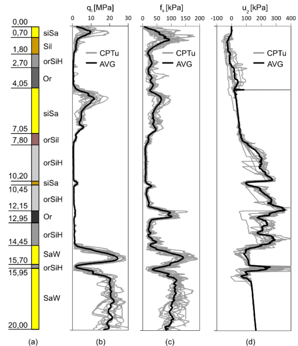
Fig. 2. Soil profile (a), and CPTU results (b)-(c) for Jazowa testing site.
