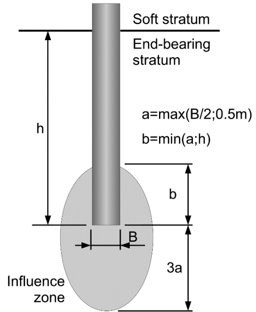
Fig. 1. Model for equivalent cone resistance ( q_{ce} ) determination.
