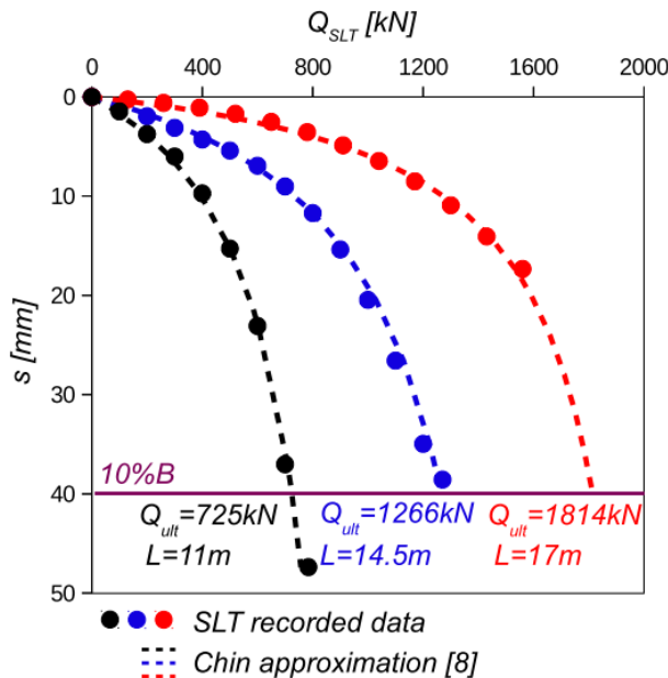
Fig. 3. Results of static load test for Jazowa reference columns.
