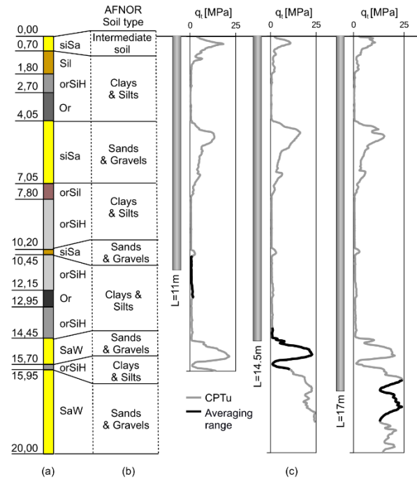
Fig. 4. Averaging depths for equivalent cone resistance determination for Jazowa reference piles.
