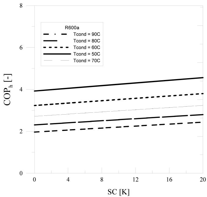
Figure 9: COPh for R600a, with variable subcooling
