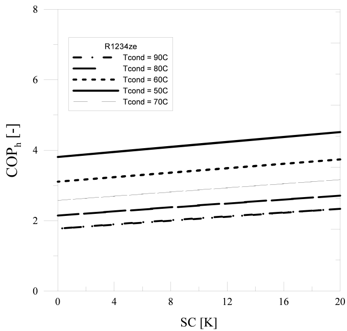
Figure 8: COPh for R1234ze, with variable subcooling
