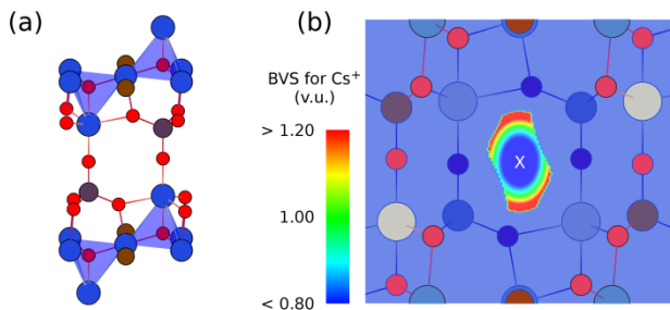
Figure 4 (a) The copper oxyphosphate framework of (\text{CsX})\text{Cu}_5\text{O}_2(\text{PO}_4)_2 . (b) Map of the bond valence sum (BVS; given in valence units – v.u.) calculated for \text{Cs}^+ cation within the unit cell. White X symbol marks the idealized (0,0, \frac{1}{2}) position, at which the deviation between BVS and the actual valence is larger than 20%. The lowest deviation (and therefore a potential energy minimum 34 ) is found off the idealized position, which is in line with the double-well site potential and observed disorder. Calculations were done using the softBV set of parameters 35 .
