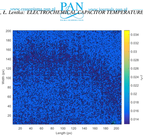
Fig. 5. A variance image of the observed surface of tested electrochemical capacitors without performing the charging/discharging processes.
