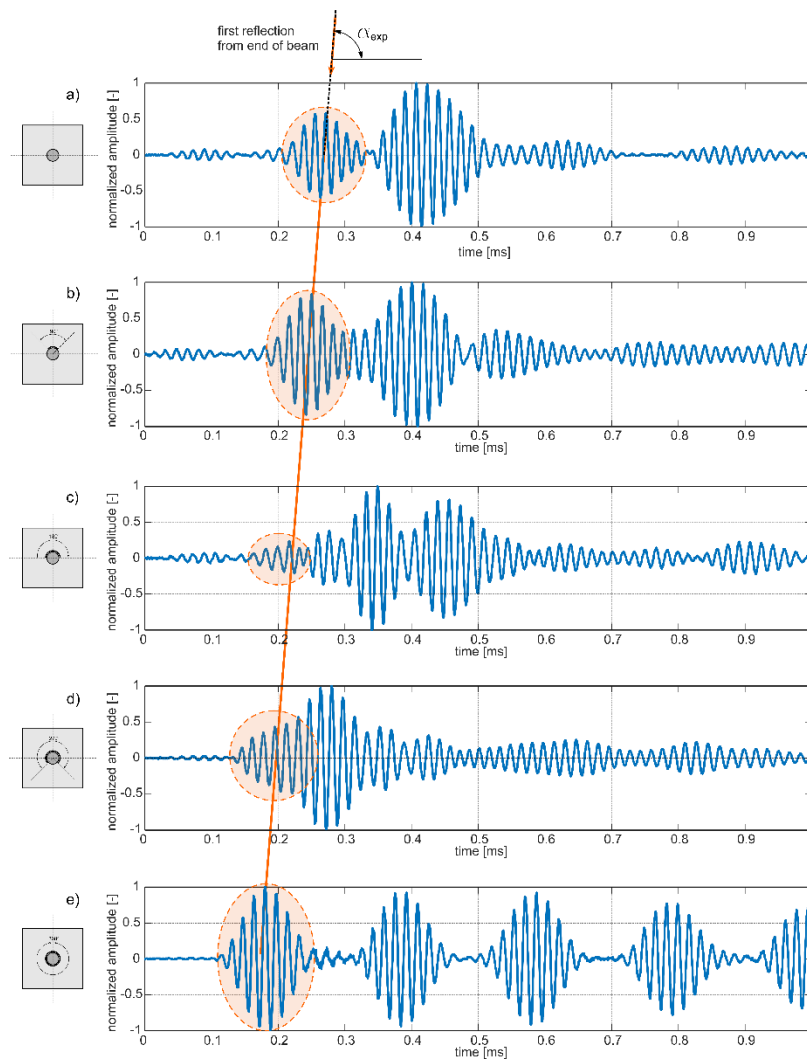
Figure 7. Experimental wave propagation signals registered at the end of the beam with variable circumferential debonding extent: (a) undamaged beam and beam with debonding extent of (b) 90°, (c) 180°, (d) 270°, and (e) 360° for excitation frequency 60 kHz.
