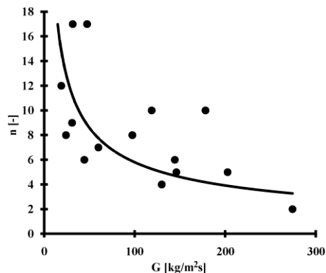
Fig. 10. Number of permanent blocked channels as a function of mass flux.
