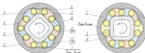
Fig.3. The working mechanism of a satellite pump [20,22-28]: C – curvature, R – rotor, S – satellite, 1÷10 – working chambers, LPC – low pressure working chamber, HPC – high pressure working chamber, V_{k-min} – working chamber with minimum area A_{min} (dead chamber), V_{k-max} – working chamber with maximum area A_{max}
