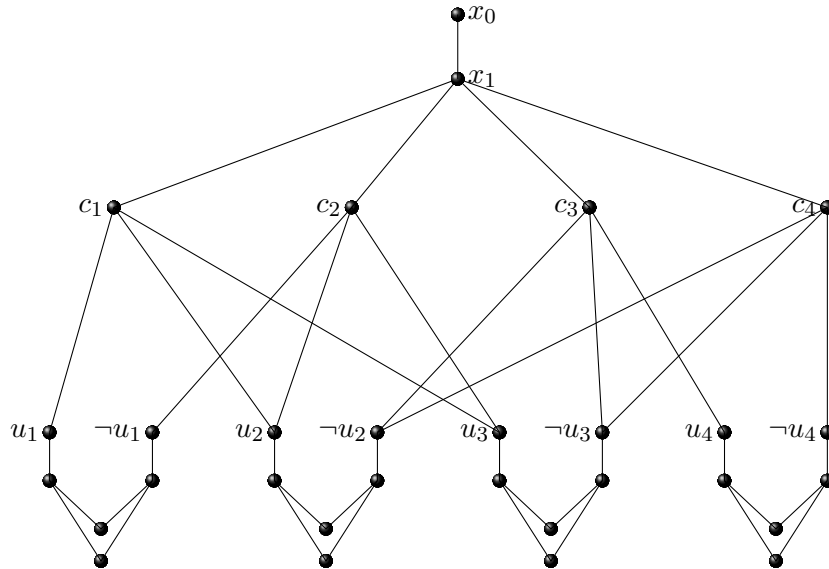
Figure 2. A construction of G for (u_1 \vee u_2 \vee u_3) \wedge (\neg u_1 \vee u_2 \vee u_3) \wedge (\neg u_2 \vee \neg u_3 \vee u_4) \wedge (\neg u_2 \vee \neg u_3 \vee \neg u_4) .
