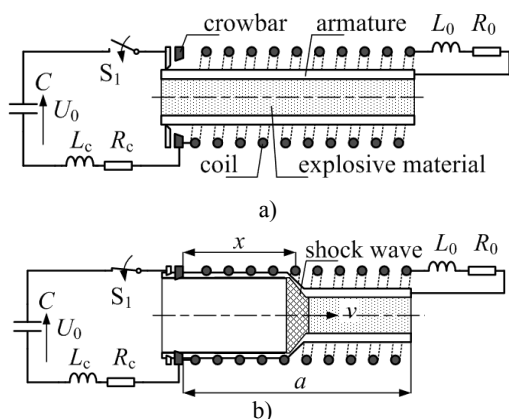
Fig. 1. FCG operation idea: a) the initial state of the system, b) magnetic field compression caused by the armature expansion process, C - capacitor bank charged to the voltage U_0 , L_c, R_c - connections inductance and resistance, L_0, R_0 - load coil inductance and resistance.
