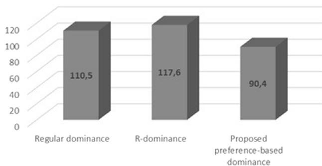
Fig. 32. Comparison of average MEWRA execution time (in seconds) in Scenario 1 with regular dominance, r -dominance and proposed preference-based dominance.
