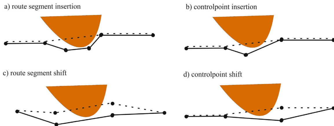
Fig. 3. Examples of problem-dedicated operators, which modify a route.
