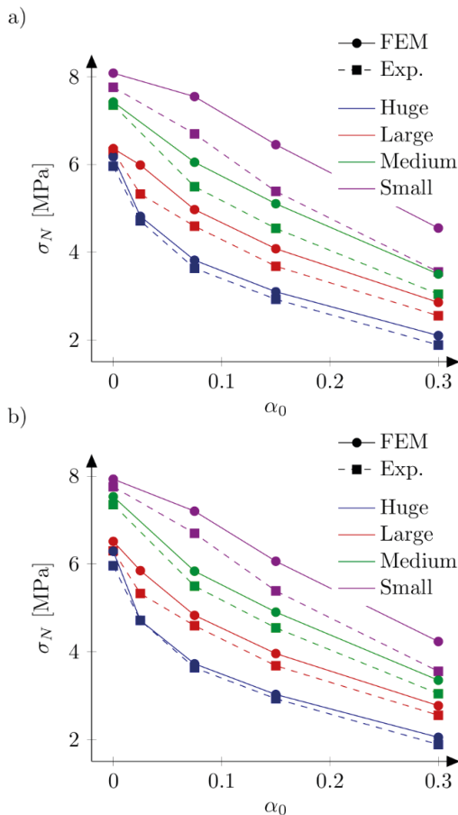
Fig. 8. Nominal (elasto-plasticity calculations) and experimental strengths with the bilinear softening curve, f_t=5.0 MPa, G_f=48 N/m and the characteristic length l=5 mm (a) and l=2 mm (b)
