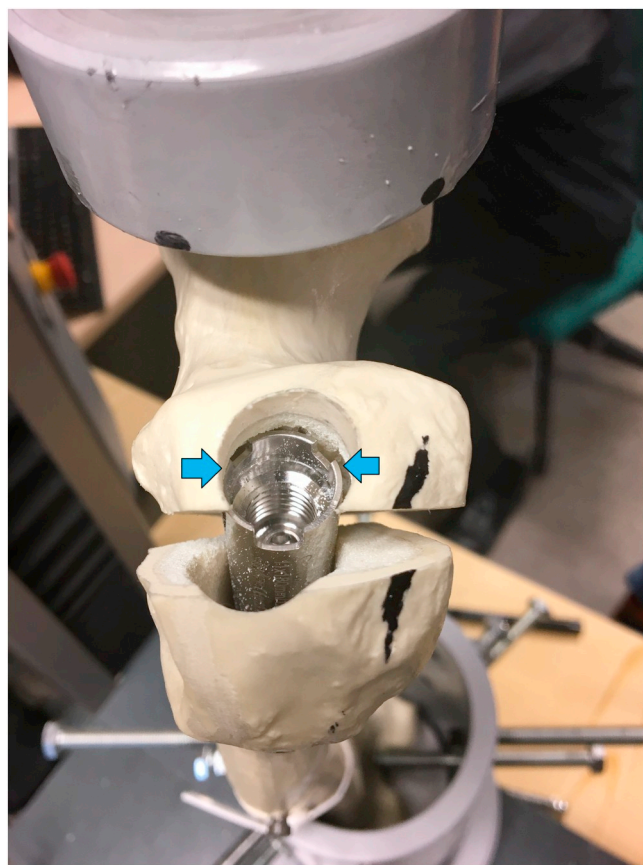
Fig. 3. The gamma nail under axial loading. The arrows show the groove in the bone that protects from rotation of the proximal fragment.
