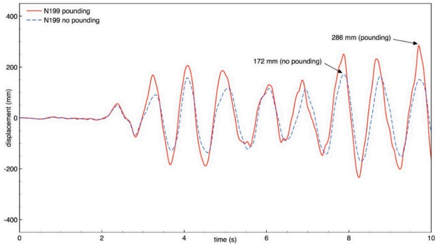
Figure 13. Longitudinal response of building A (node N199) with and without pounding.
