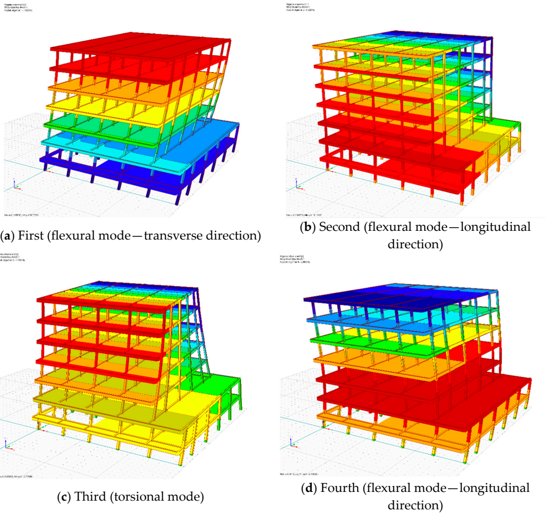
Figure 6. Modes of free vibrations for building A.
